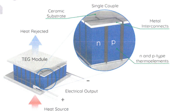
FIGURE 1. Structure of TEG consist of p-type and n-type thermoelements (Sharma et al., 2020; Shilpa et al., 2022)
