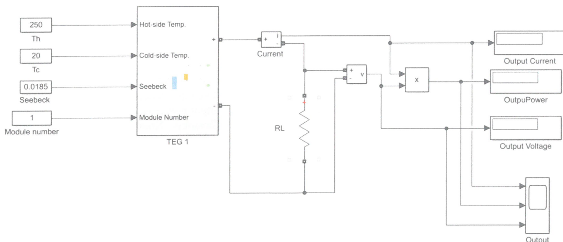
FIGURE 5. Model of TEG system using a single TEG module
