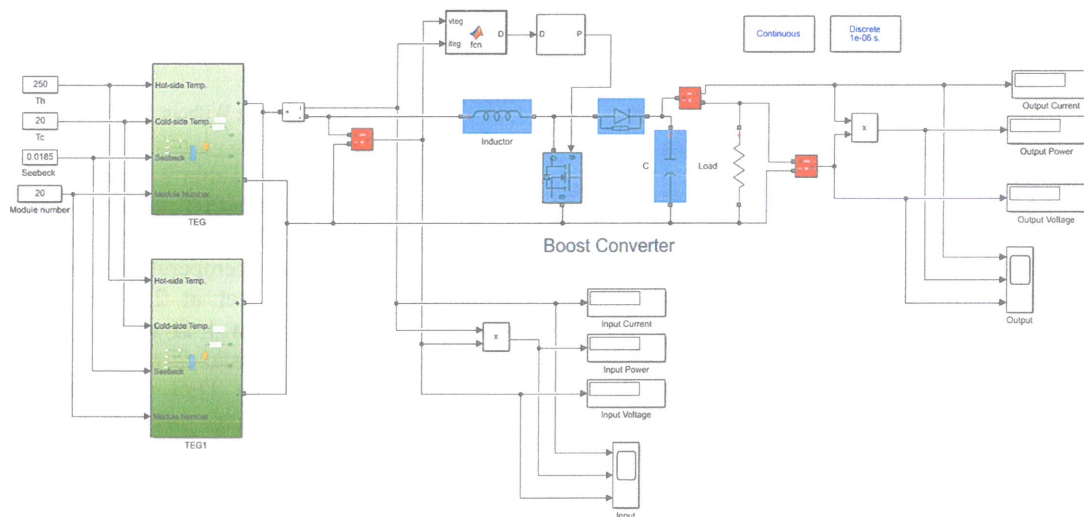
FIGURE 7. Two TEG modules connected in series-parallel combination with a P&O MPPT
