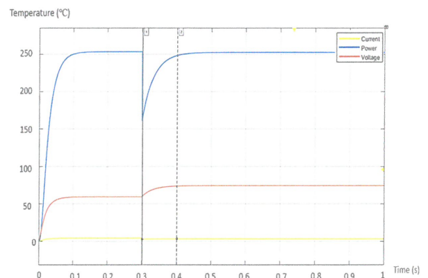
FIGURE 10. Simulation result when load changes from 7 \Omega to 15 \Omega
