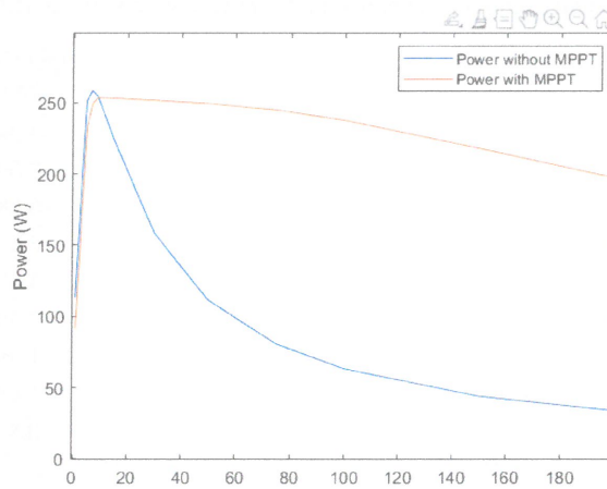
FIGURE 8. Power without MPPT and Power with MPPT graph
