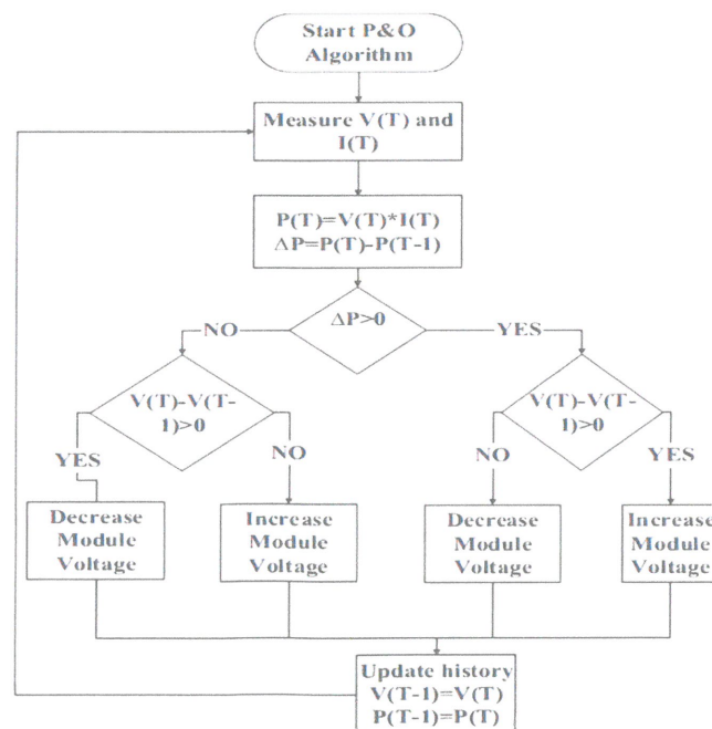
FIGURE 4. Flowchart of Perturb and Observe algorithm (El-Shahat & Bhuiyan, 2021)
