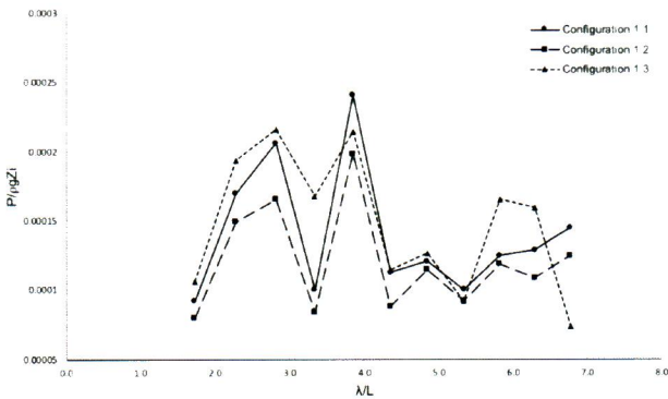
Fig. 4. Pressure Amplitude for Configuration 1
