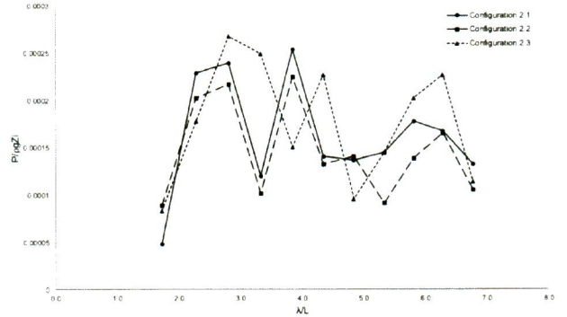
Fig. 5. Pressure Amplitude for Configuration 2
