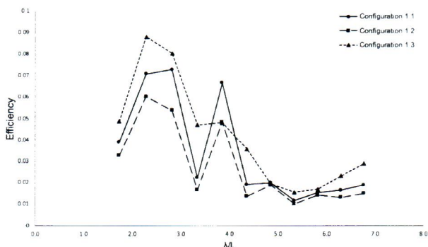
Fig. 8. Efficiency of device for Configuration 1
