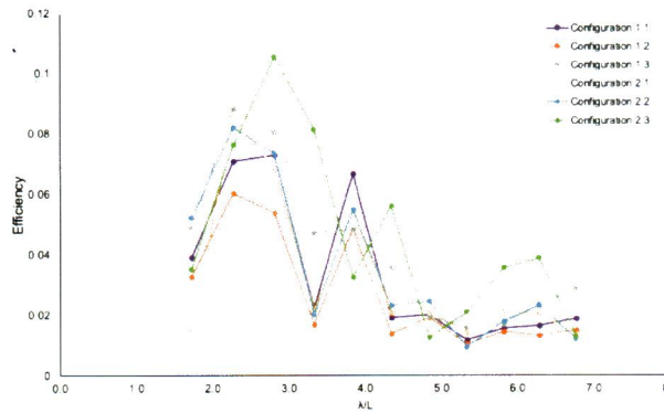
Fig. 10. Overall Efficiency of BBDB device
