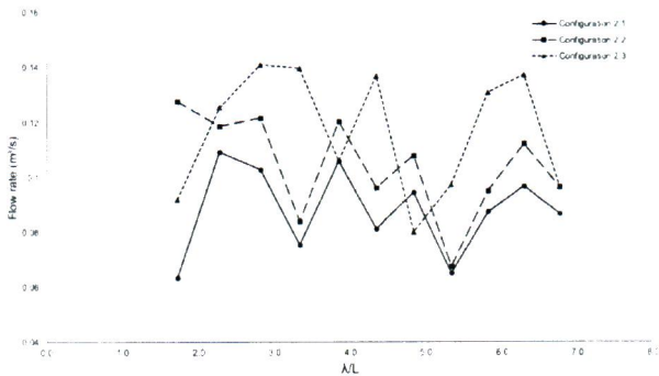
Fig. 7. Air flow rate at the orifice outlet in Configuration 2
