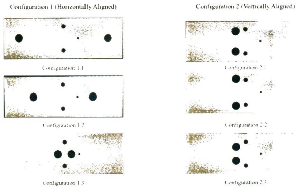
Fig. 2. Fabricated Top Panels
