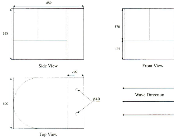
Fig. 1. Drawing of BBDB from 3 different perspective
