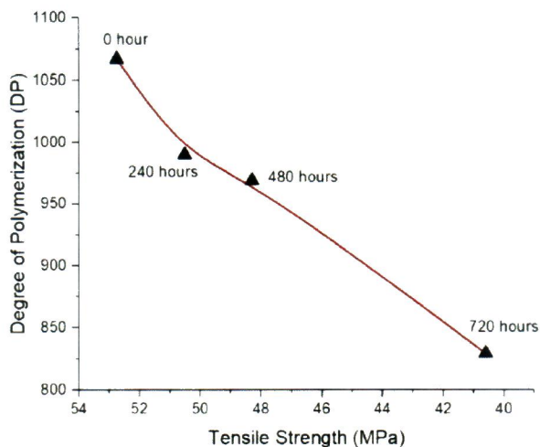
Fig. 6 Tensile Strength and Degree of Polymerization with increasing aging hours
