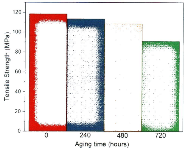
Fig. 5 Tensile Strength with increasing aging hours
