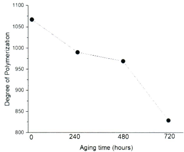
Fig. 4 Degree of Polymerization with increasing aging hours
