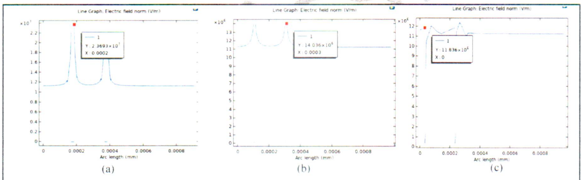
FIGURE 15. Graph of electric field recorded along a straight line in Case 2 for different shapes of alumina nanoparticle (a) sphere (b) rod (c) triangle
