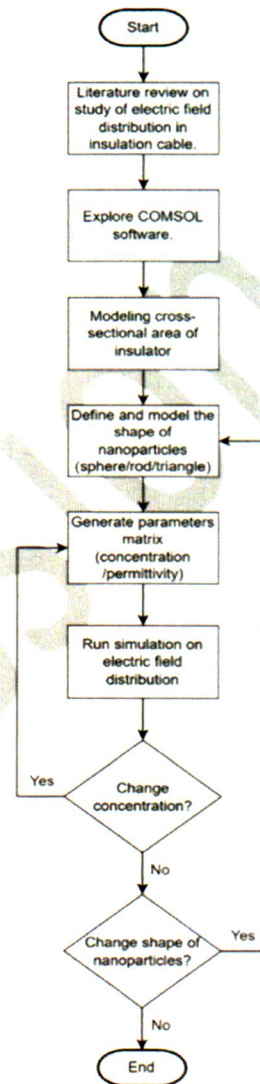
FIGURE 1. Research flowchart
