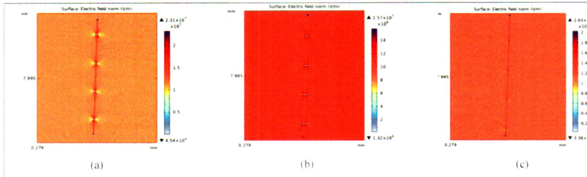
FIGURE 17. Electric field of XLPE containing 7 layers with different shapes alumina nanoparticles along a straight line (a) sphere (b) rod (c) triangle
