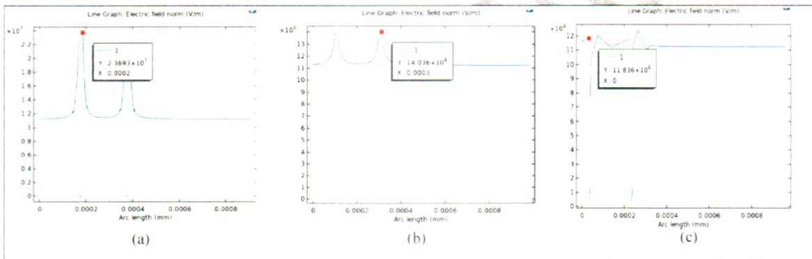
FIGURE 12. Graph of electric field recorded along a straight line in Case 1 for different shapes of alumina nanoparticle (a) sphere (b) rod (c) triangle
