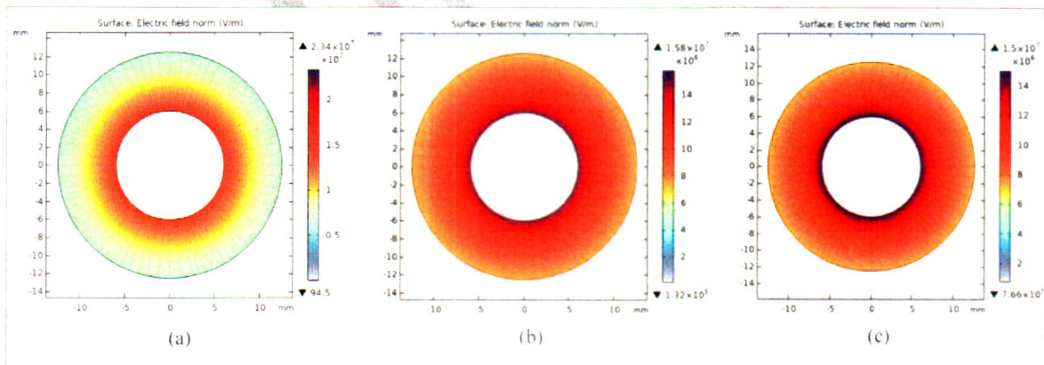
FIGURE 10. XLPE cable with different shapes of alumina nanoparticle for Case 1 (a) sphere (b) rod (c) triangle
