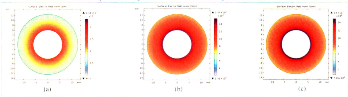
FIGURE 16. XLPE cable with different shapes of alumina nanoparticle for Case 3 (a) sphere (b) rod (c) triangle
