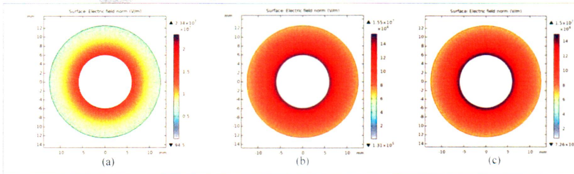
FIGURE 13. XLPE cable with different shapes of alumina nanoparticle for Case 2 (a) sphere (b) rod (c) triangle
