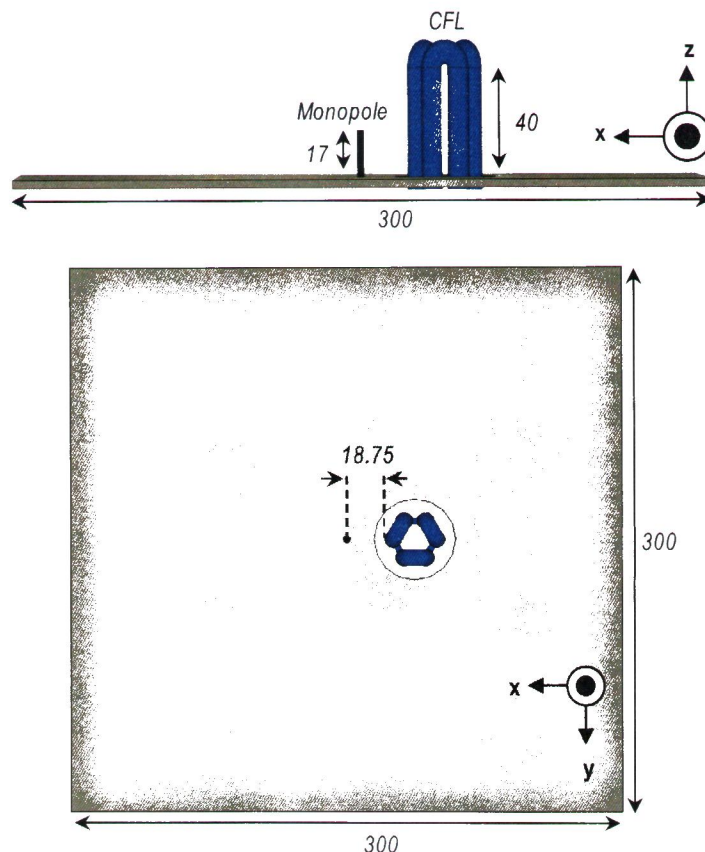
Fig. 2. Schematic diagram of antenna used for the radiation pattern measurement (Unit in mm)
