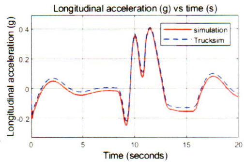
(b) Longitudinal acceleration for SLC
