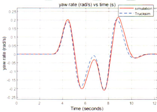
(c) Yaw rate for DLC
