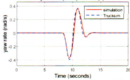
(c) Yaw rate for SLC
