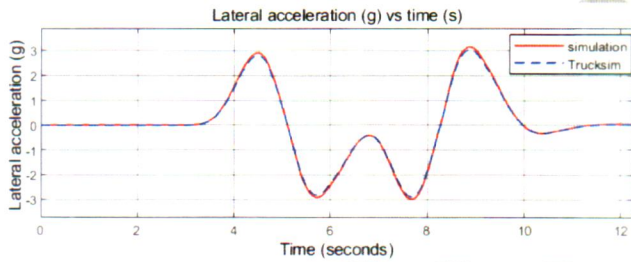
(a) Lateral acceleration for DLC
