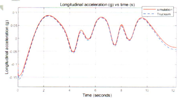
(b) Longitudinal acceleration for DLC
