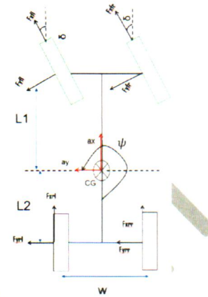
Fig.2. Handling model for bus.(Mohd Yussof et al., 2020)
