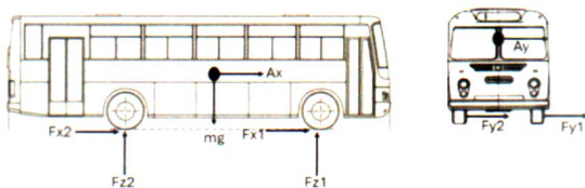
Fig.1. Side and front view of the bus model.(Sekulić, 2020)
