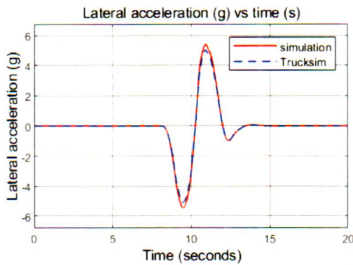
(a) Lateral acceleration for SLC
