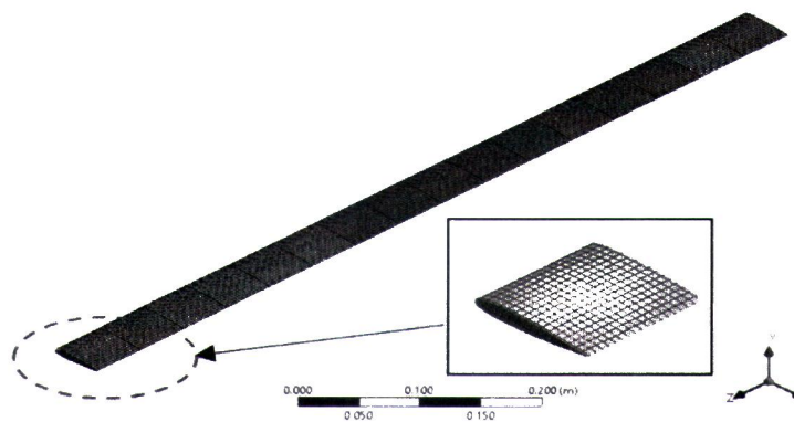
Figure 6 Structural mesh of the HAR wing model
