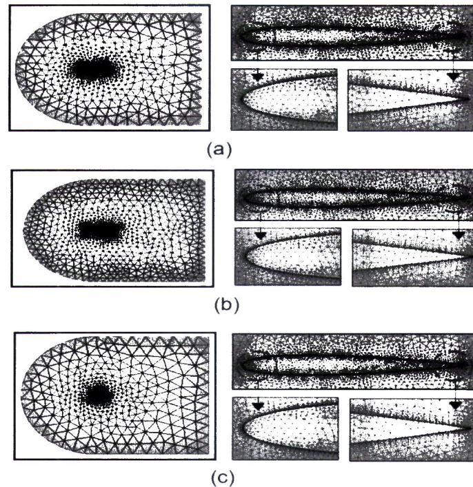
Figure 5 Meshing of the HAR wing model: (a) coarse mesh, (b) base mesh, (c) fine mesh
