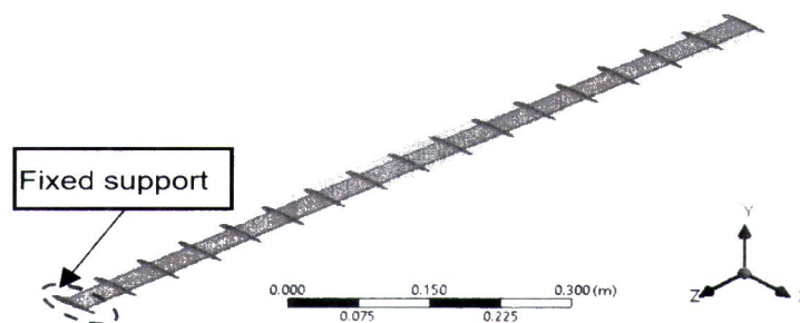
Figure 7 Boundary condition for HAR wing model
