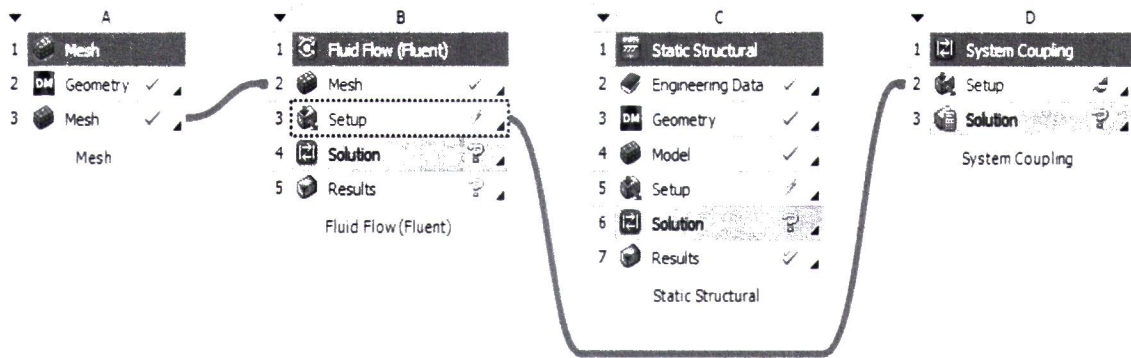
Figure 9 Coupling system for two-way FSI analysis
