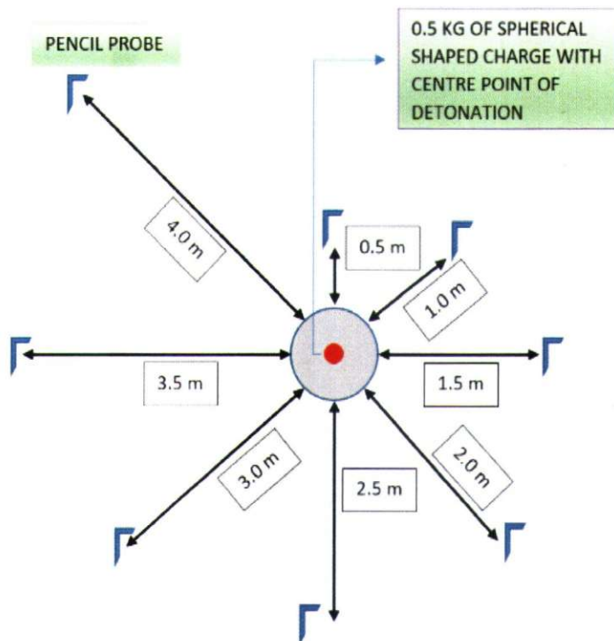
Fig. 10. Field blast test set up.
