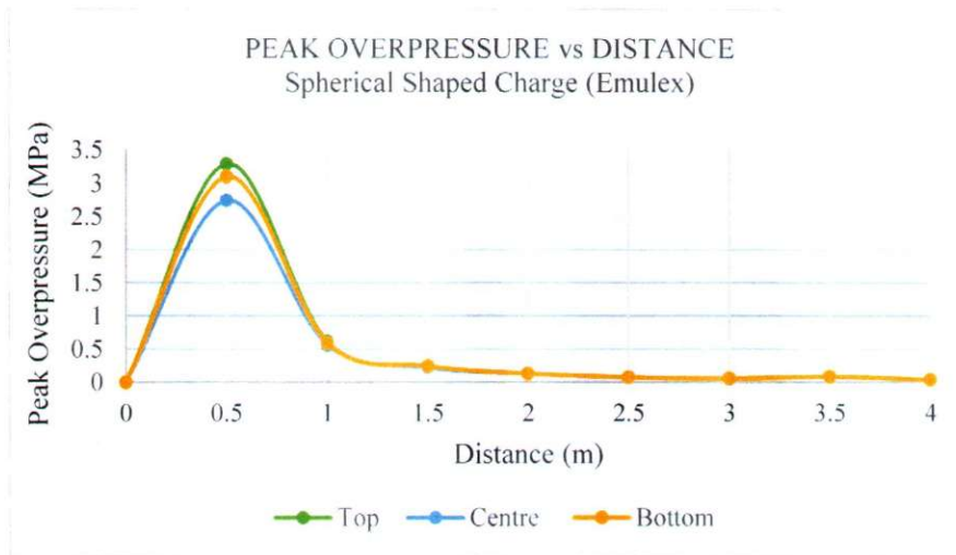
Fig. 11. Peak overpressure for emulsion explosive over the distance from 0.5 m to 4.0 m.
