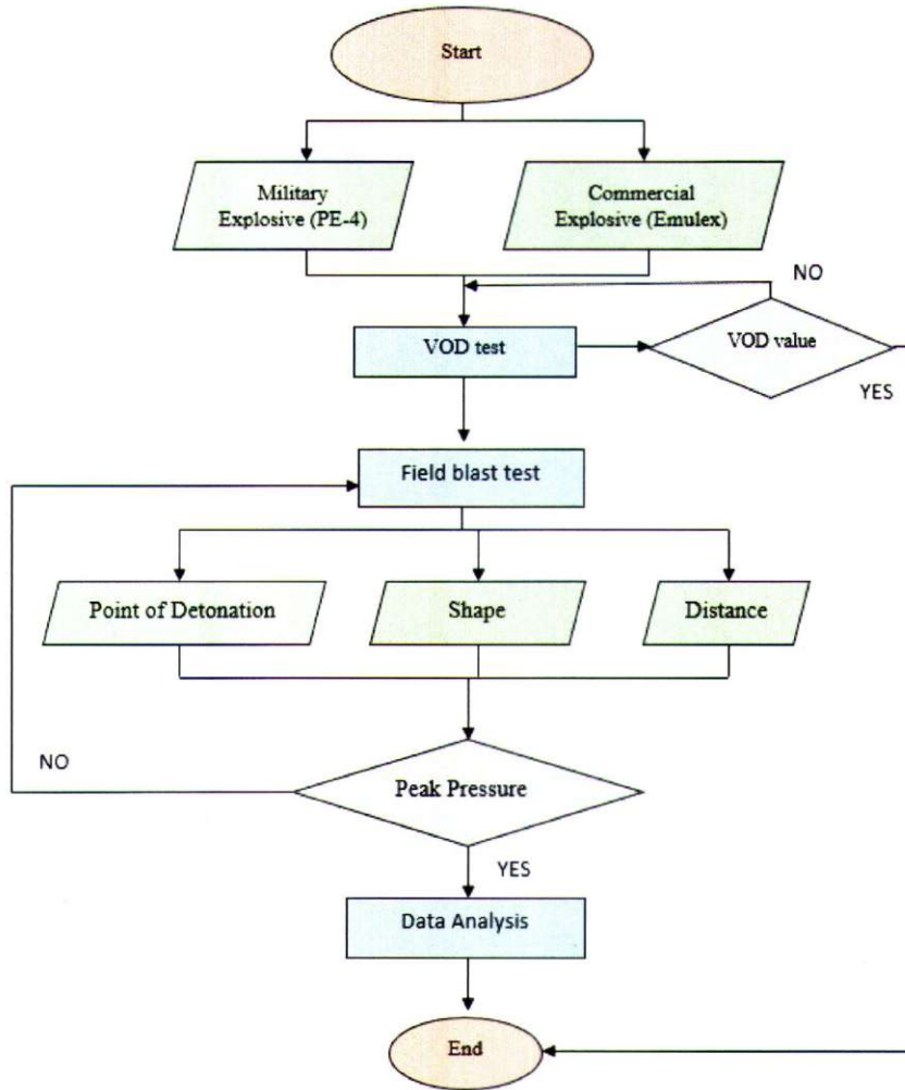
Fig. 7. Experimental flow chart.
