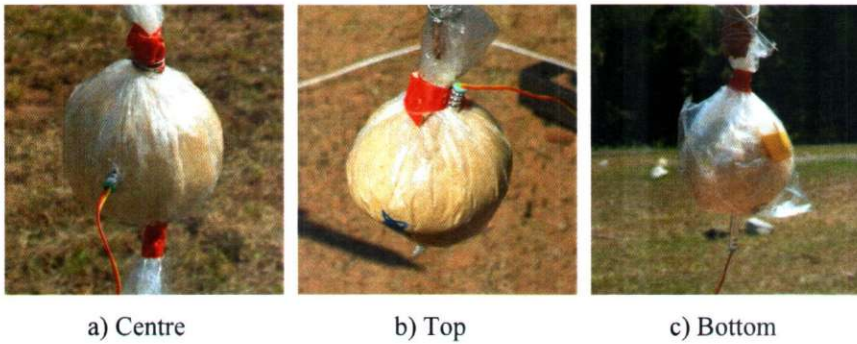
Fig. 9. The point of initiation for spherical charge of explosive.
