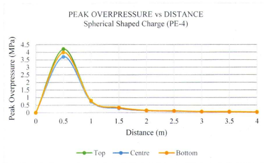
Fig. 12. Peak overpressure for PE-4 over the distance from 0.5 m to 4.0 m.
