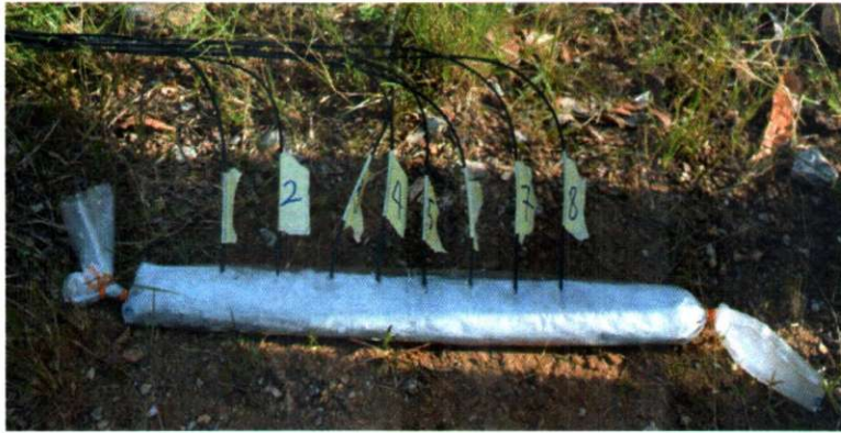
Fig. 8. Detonation velocity testing using fiber optic cables [2].
