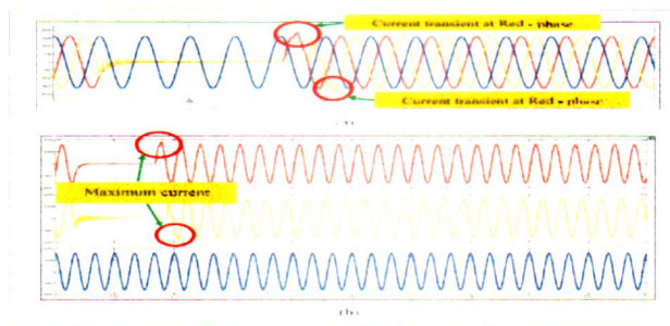
FIGURE 9. (a) Output current (b) R – Y – B output voltage LL - G fault current LL - G fault.
