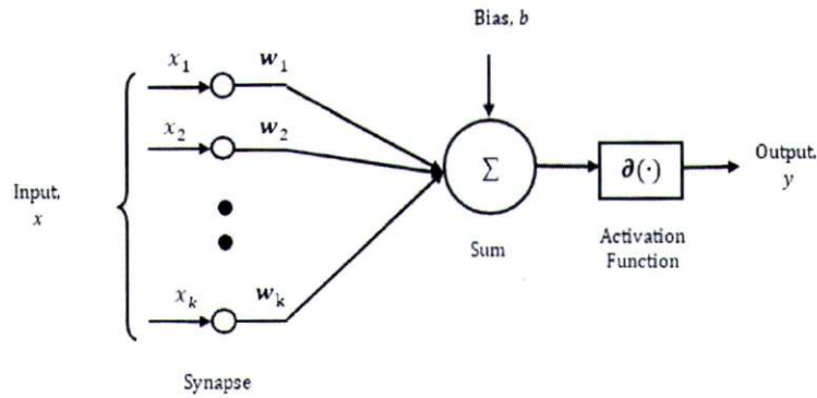
Fig. 3. Nonlinear neuron model [18].
