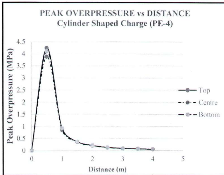
Fig. 5. The recorded data during the explosive testing.
